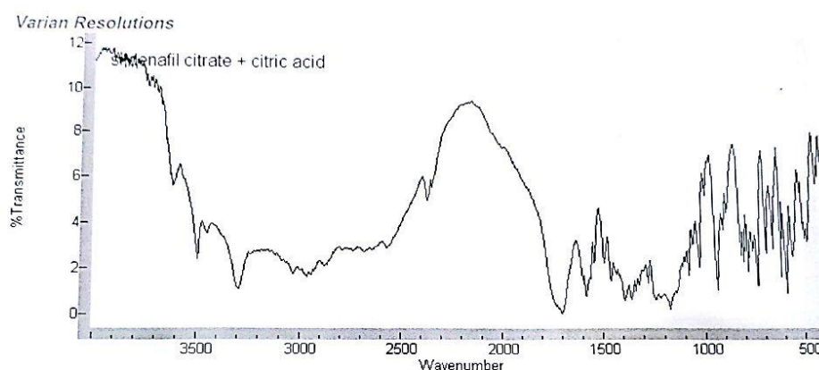
Fig. 8: FTIR Spectrum of Physical Mixture of Sildenafil Citrate and Citric Acid.
