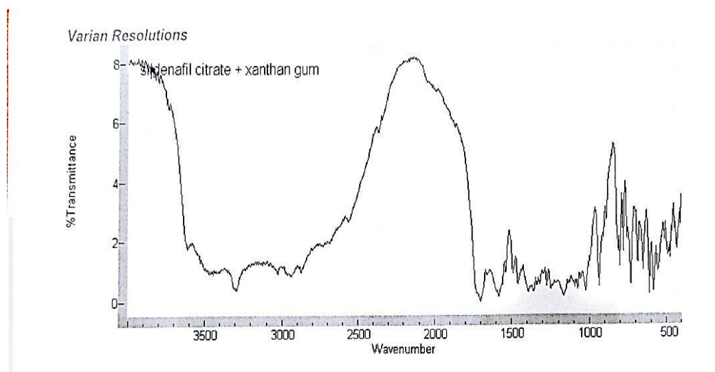
Fig. 4: FTIR Spectrum of Physical Mixture of Sildenafil Citrate and Xanthan Gum.
