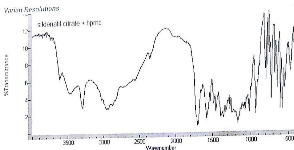
Fig. 5: FTIR Spectrum of Physical Mixture of Sildenafil Citrate and HPMC.
