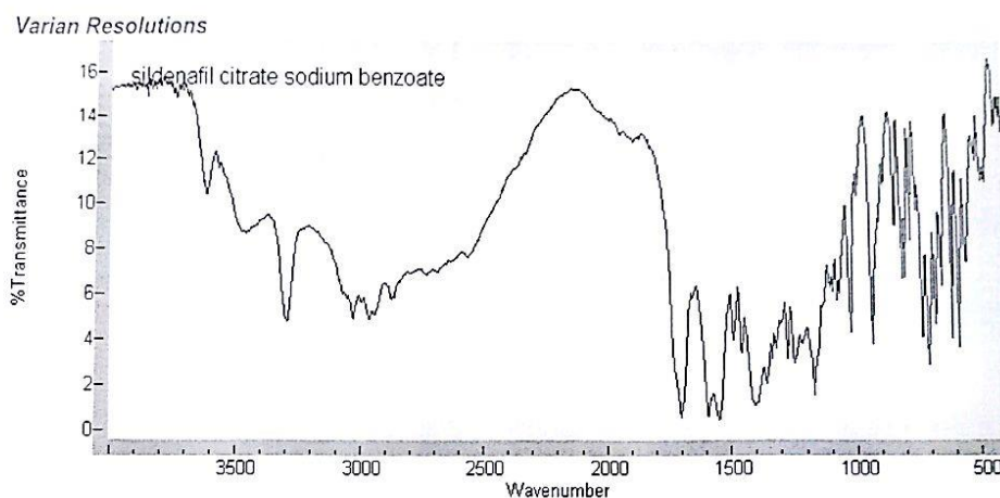
Fig. 7: FTIR Spectrum of Physical Mixture of Sildenafil Citrate and Sodium Benzoate.
