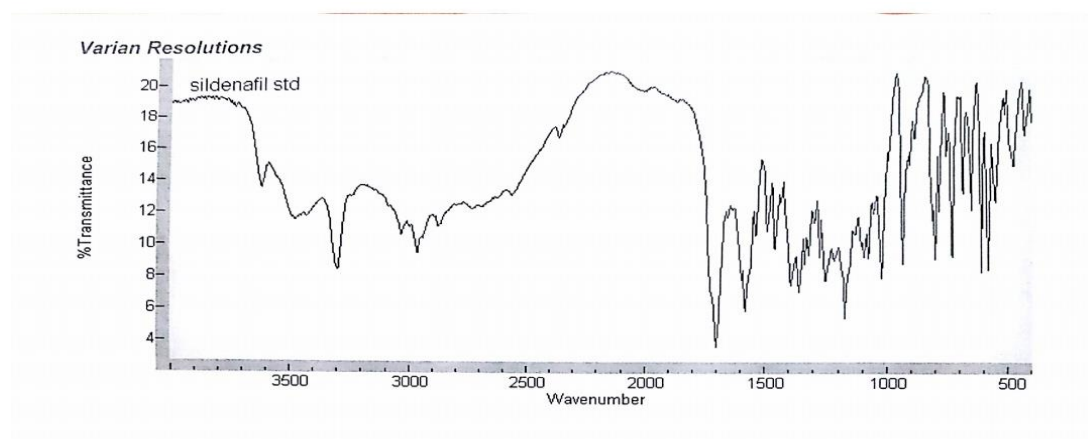
Fig. 2: FTIR Spectrum of Standard Sildenafil Citrate.
