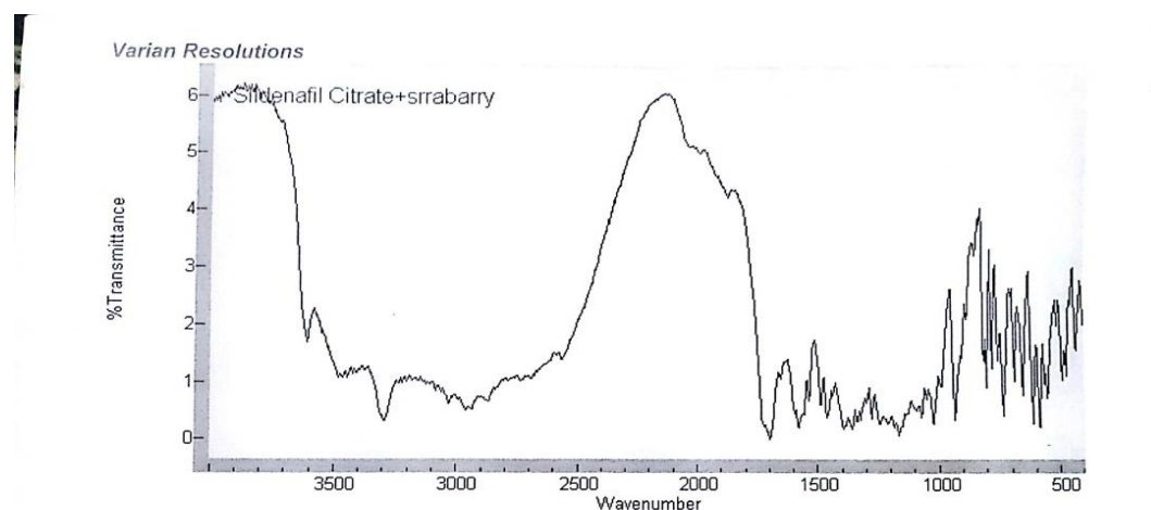
Fig. 13: FTIR Spectrum of Physical Mixture of Sildenafil Citrate and Strawberry.
