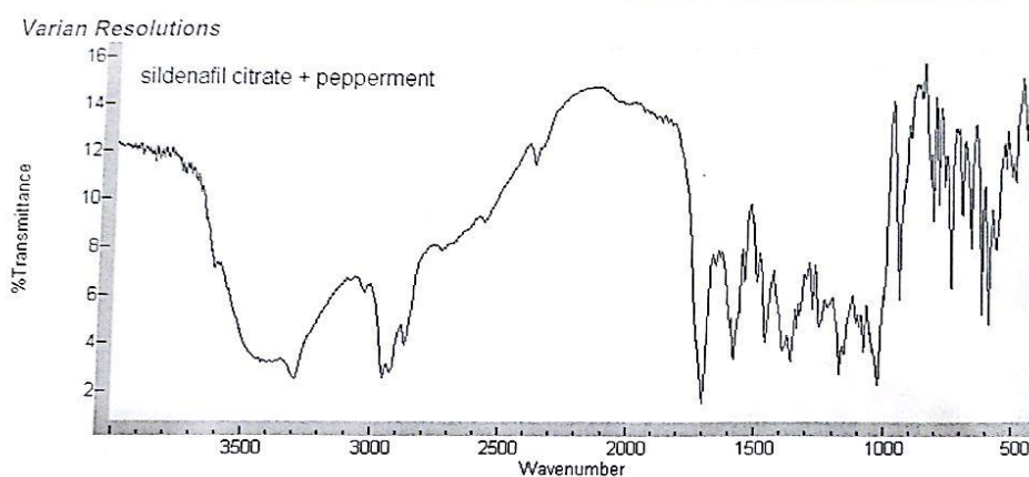
Fig. 12: FTIR Spectrum of Physical Mixture of Sildenafil Citrate and Peppermint.
