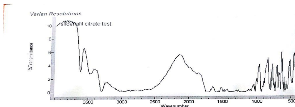
Fig. 3: FTIR Spectrum of Standard Sildenafil Citrate and Sildenafil Citrate.
