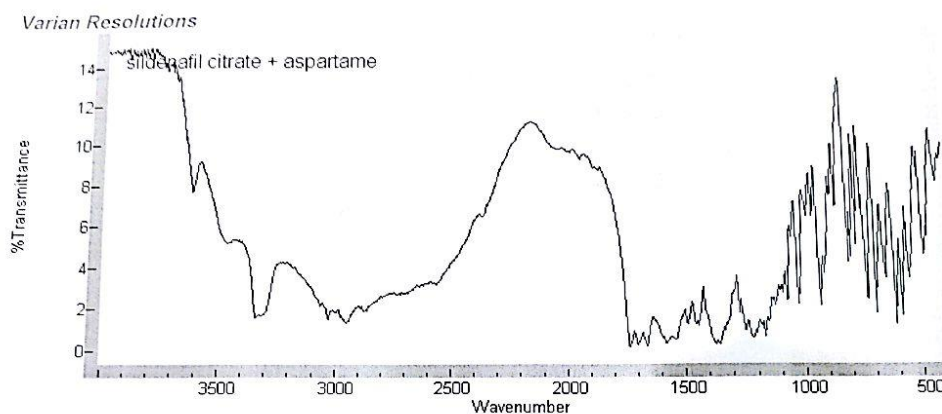
Fig. 10: FTIR Spectrum of Physical Mixture of Sildenafil Citrate and Aspartame.
