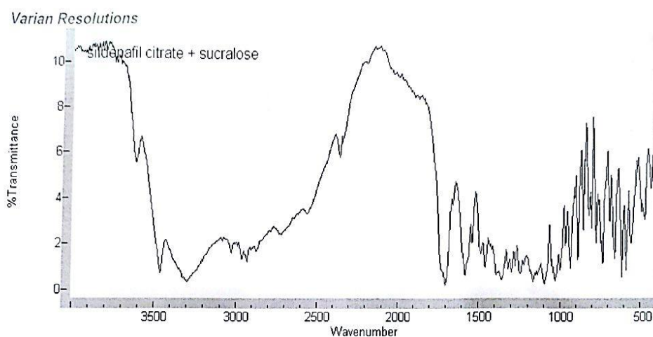
Fig. 9: FTIR Spectrum of Physical Mixture of Sildenafil Citrate and Sucralose.
