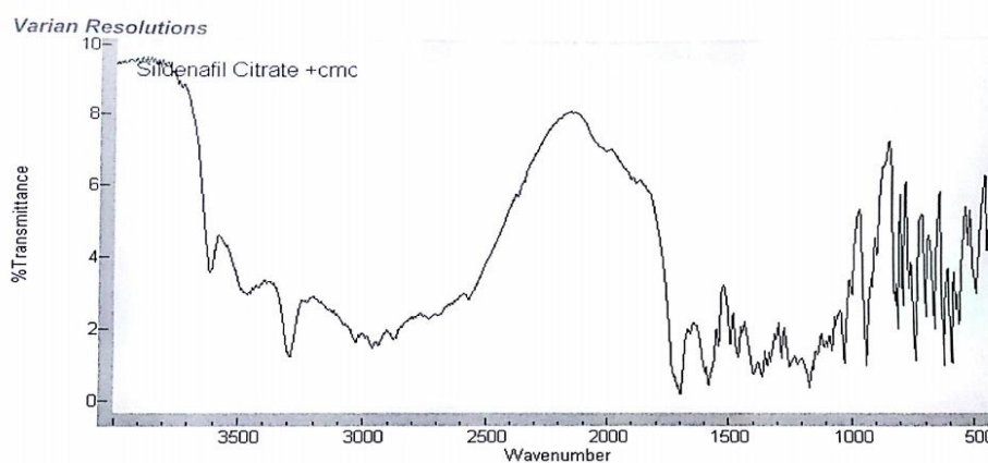
ig. 6: FTIR Spectrum of Physical Mixture of Sildenafil Citrate and CMC.
