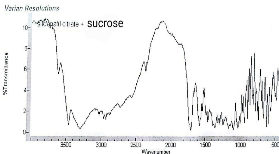
Fig. 11: FTIR Spectrum of Physical Mixture of Sildenafil Citrate and Sucrose.
