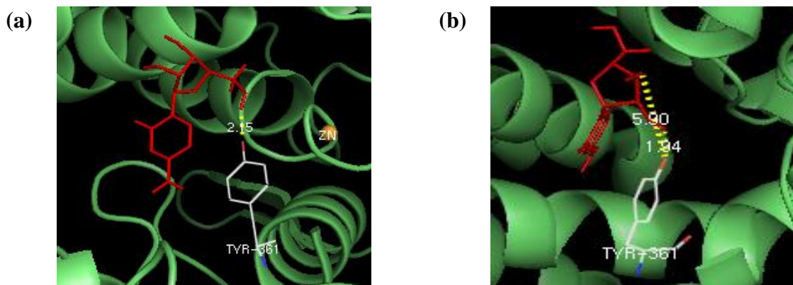
Figure 1(a-b): The docking structure of complex between Farnesyltransferase and inhibitor Azacitidine (a) with Zinc and (b) without Zinc. Inhibitor Azacitidine is show in sticks representation and is colored with red using PyMol viewer. Amino acid residues are represented as lines. Hydrogen bond is represented by yellow dotted line.
