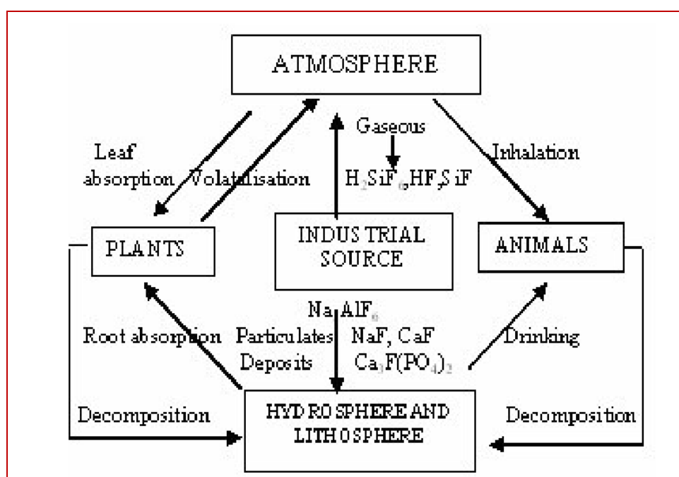
Figure 1. Fluoride cycle in the environment of Nalco
