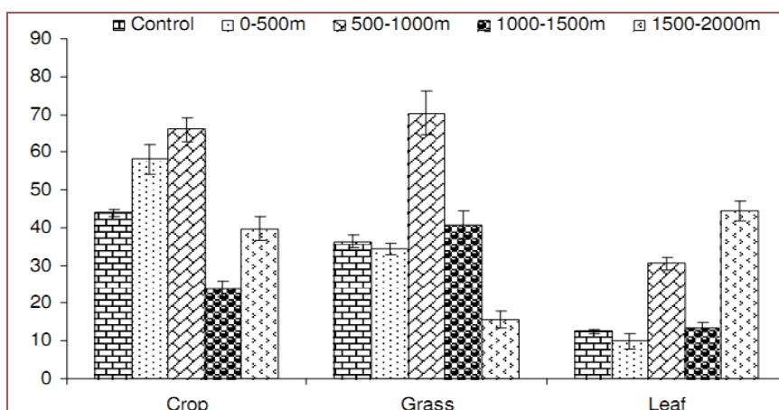
Figure 4. Variation in fluoride (mg/kg) content in Crop, Grass and Leaf samples in control and experimental site (Mean \pm SD).
