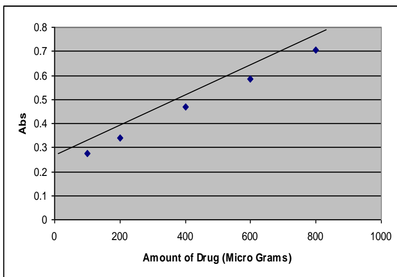
Figure 3: calibration curve for Gatifloxacin
