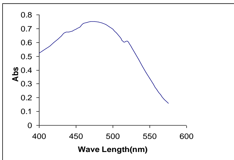
Figure 2: Spectrum of gatifloxacin
