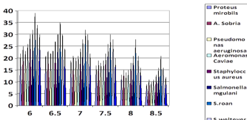
Fig. 10: pH Effect of pH on the antimicrobial activity of allicin.
