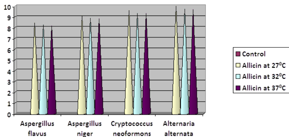
Fig. 2: Antifungal Activity of Allicin against different fungus at 0.55%.
