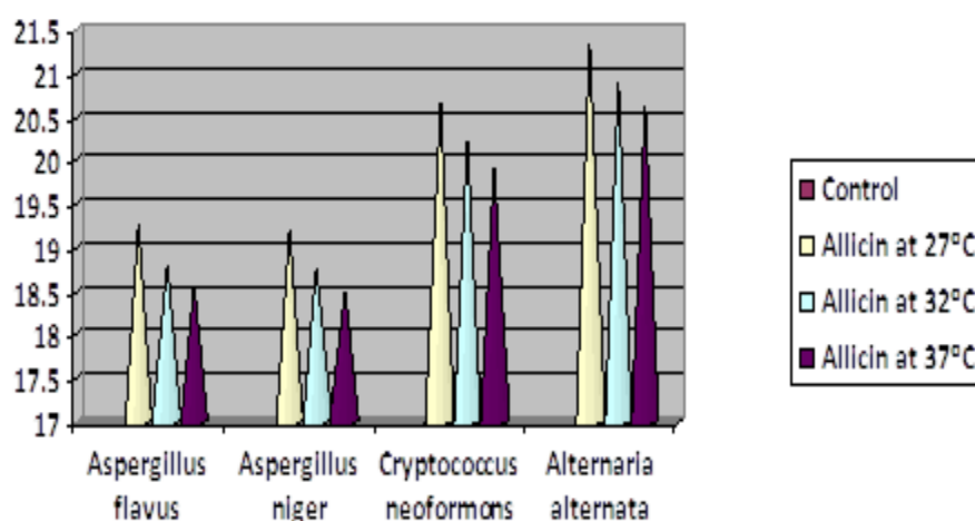
Fig. 6: Antifungal Activity of Allicin against different fungus at 0.95 %.
