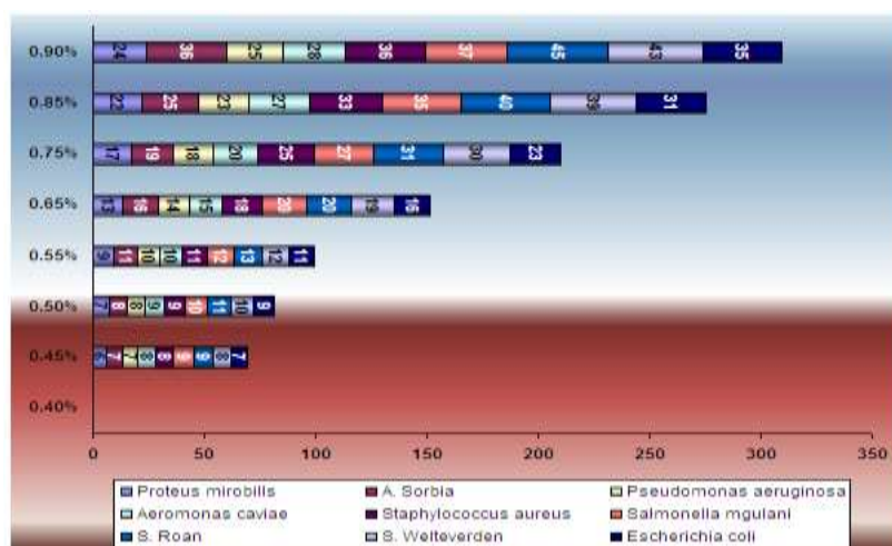
Fig. 8: Antibacterial Activity of Allicin against different bacteria at different conc. At 32°C.
