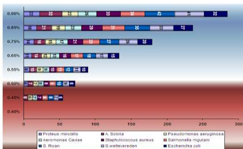
Fig. 9: Antibacterial Activity of Allicin against different bacteria at different conc at 37°C.
