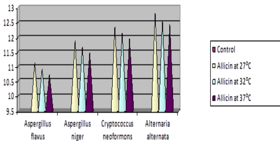
Fig. 3: Antifungal Activity of Allicin against different fungus at 0.65 %.
