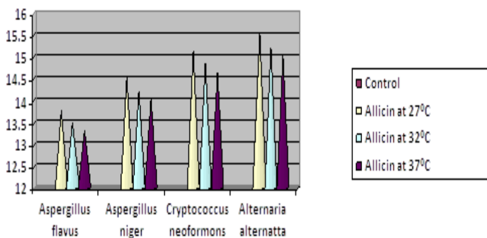
Fig. 4: Antifungal Activity of Allicin against different fungus at 0.75 %.
