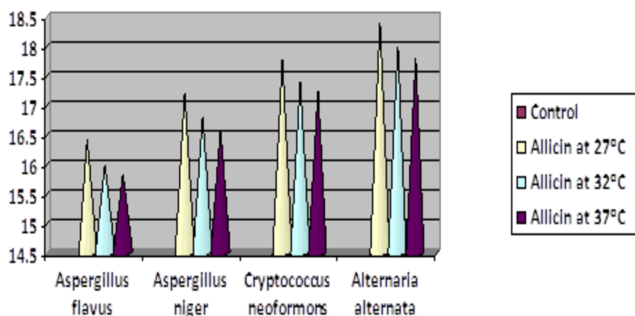
Fig. 5: Antifungal Activity of Allicin against different fungus at 0.85 %.
