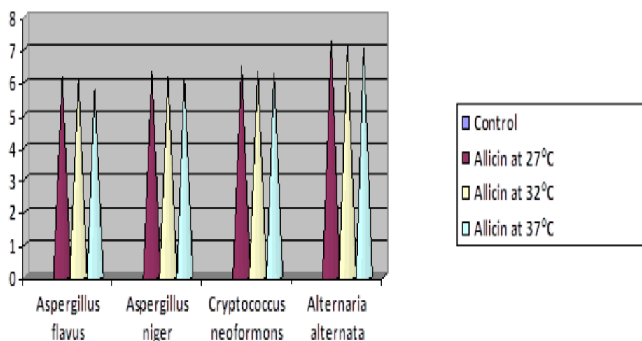
Fig. 1: Antifungal Activity of Allicin against different fungus at 0.45 %.
