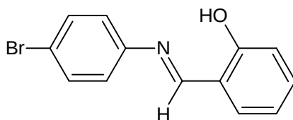
Figure 1. Primary ligand: 2-[(E)-[(4-bromophenyl)imino]methyl]phenol.
