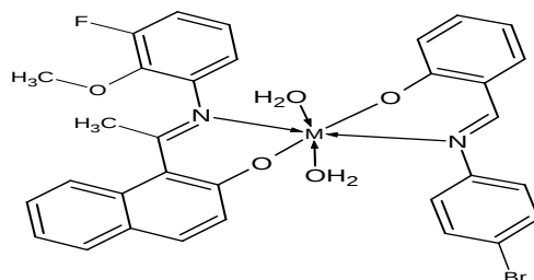
Figure 4. The metal-ligand ternary binding proposed structure.
