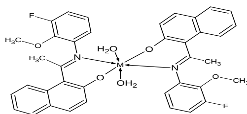
Figure 3. The metal-ligand binary binding proposed structure.
