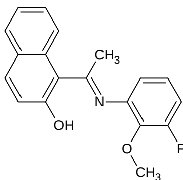
Figure 2. Secondary ligand: 1-[(1E)-N-(3-fluoro-2-methoxyphenyl) ethanimidoyl] naphthalen-2-ol.
