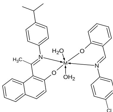
Figure 4: The metal-ligand ternary binding proposed structure.
