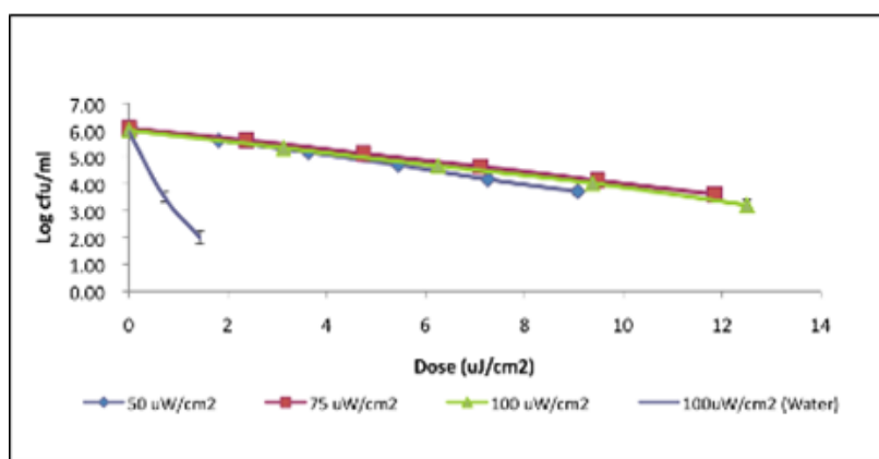
Figure 3-4: Inactivation of Bacillus subtilis spores PS361 (SASP mutant) in 10mg/ml skim milk or water at different UV intensities such as 50, 75 and 100 \mu\text{W}/\text{cm}^2 .
