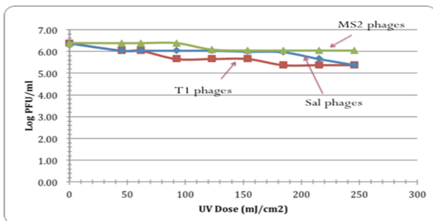
Figure 3-8: UV inactivation kinetics of bacteriophages (T1, Sal, and MS2 phages) in collimated beam UV apparatus in skim milk (10% w/v) at 50\mu\text{W}/\text{cm}^2 UV intensity.
