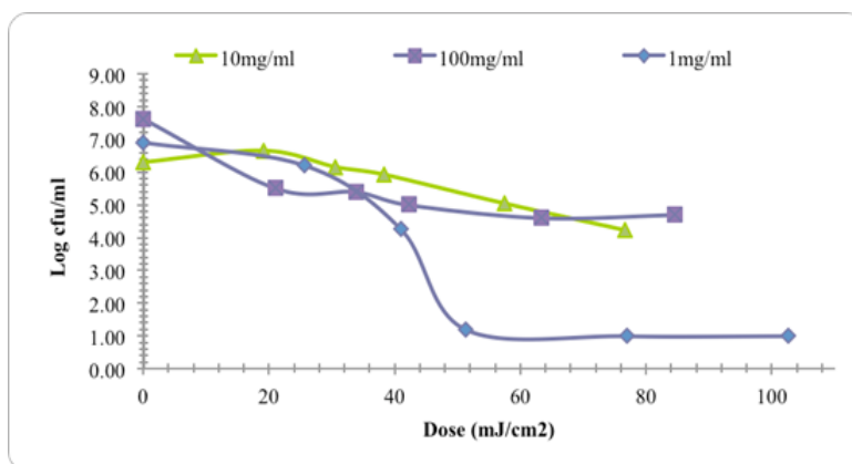
Figure 3-3: Inactivation kinetics of Bacillus subtilis spores PS346 in skim milk with different concentrations of skim milk such as 1mg/ml, 10mg/ml, and 100mg/ml (w/v) at 100 \mu\text{W}/\text{cm}^2 UV intensity.
