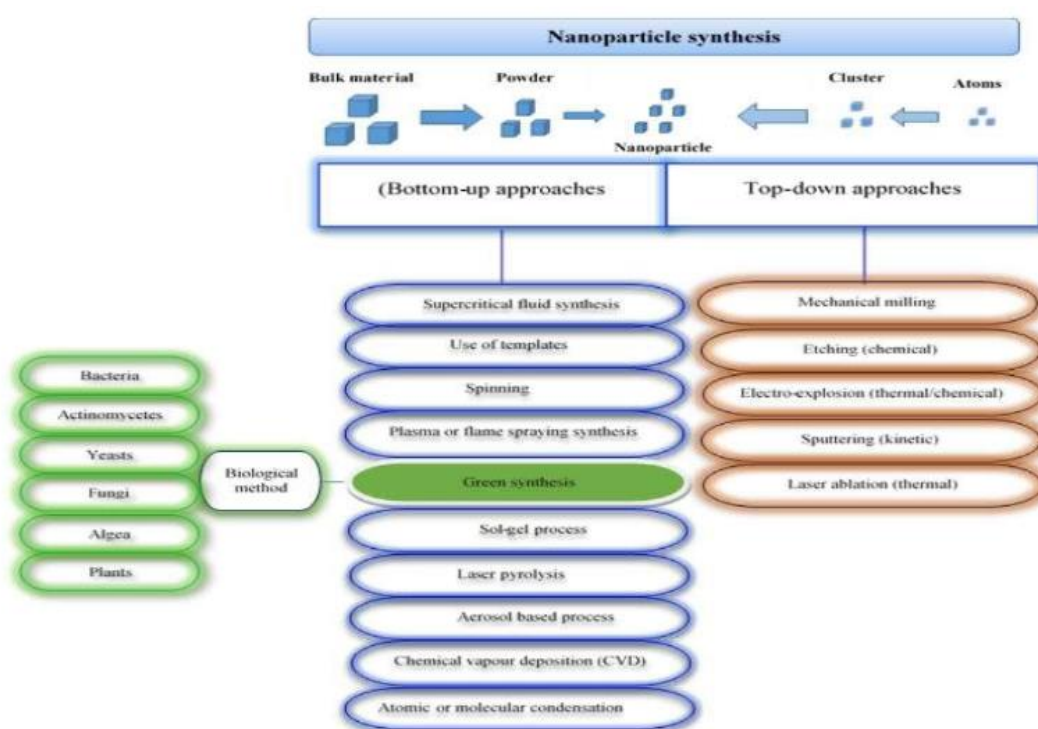
Figure 2: Synthesis methods of N Ps. [10]
