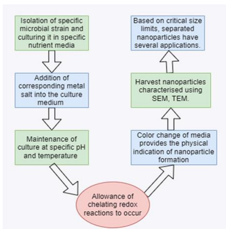
Figure 4: General mechanism for microorganismal-based NP synthesis.
