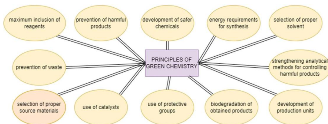
Figure 1: Fundamentals/Principles of Green Chemistry.
