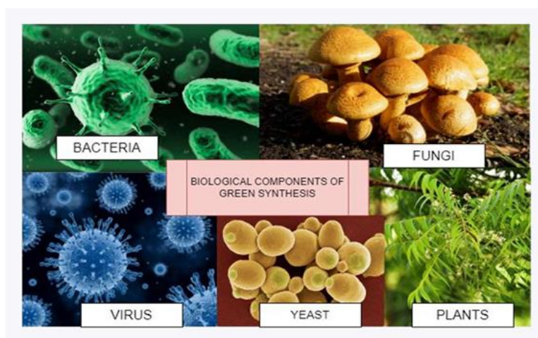
Figure 3: Biological Components of Green Synthesis.
