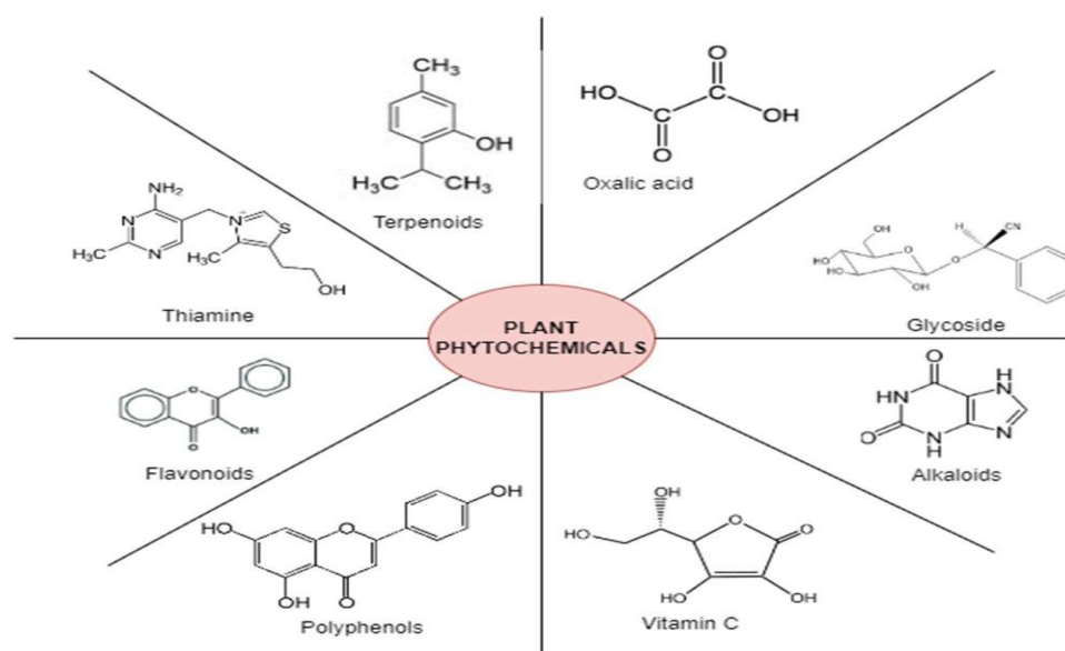
Figure 6: Phytochemicals present in plants.
