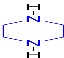
Figure 1: Piperazine.
