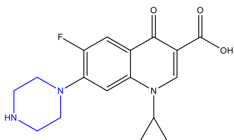
Figure:- 2 Ciprofloxacin
