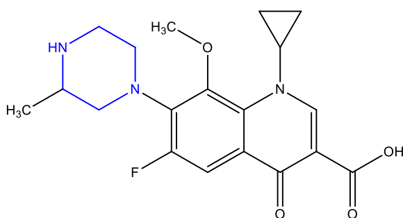
Figure:-4 Gatifloxacin
