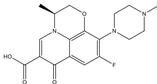
Figure:-7 Levofloxacin
