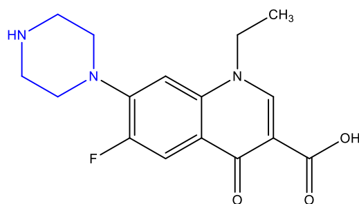
Figure:-3 Norfloxacin
