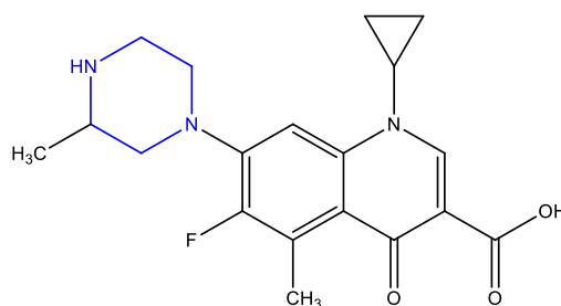
Figure:-5 Grepafloxacin
