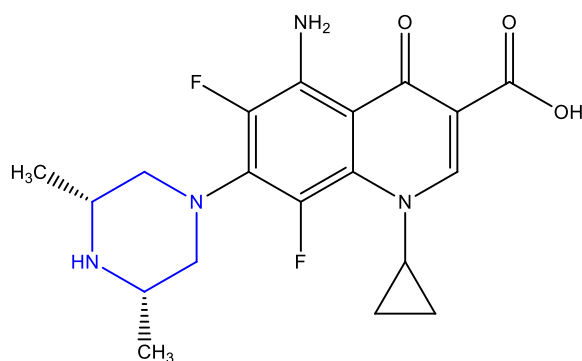
Figure:-6 Sparfloxacin
