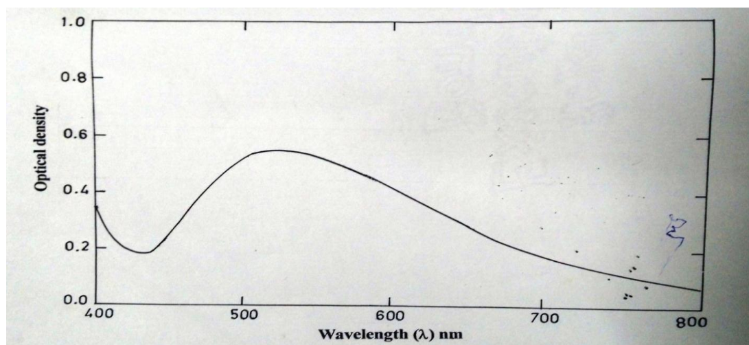
Fig 1: Charge Transfer Spectra of PQ-L-Dopa.
