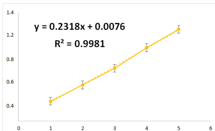
Figure No. 3: Calibration curve of silymarin in methanol.
