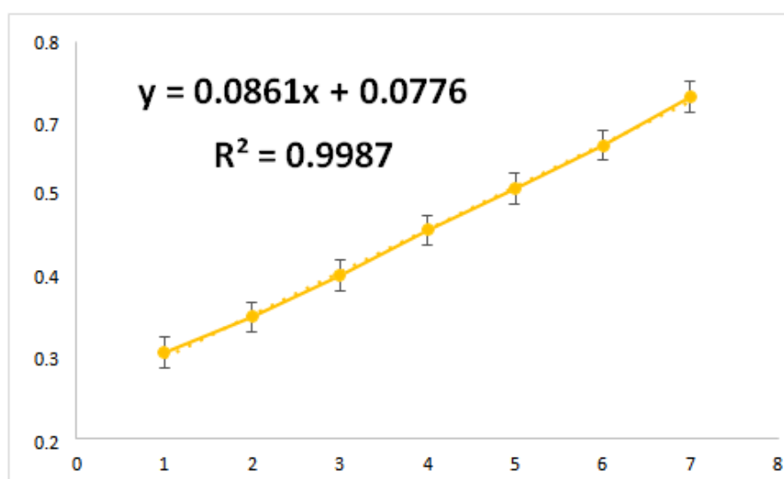
Figure No. 2: Calibration curve of rutin in methanol.
