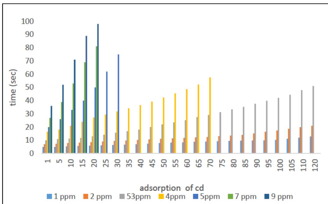
Figure 11c: Use of Fe 3 O 4 nanoparticles for removal of toxic Cd precipitated as CdS for 1-9 ppm solutions.
