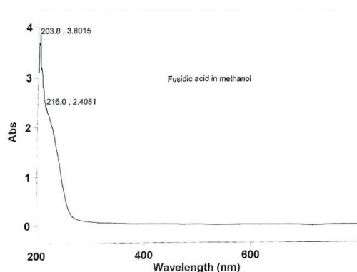
Fig. 1: Wavelength of Fusidic Acid in UV Spectrophotometer.
