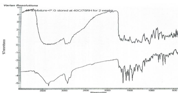
Fig. 11: FTIR Spectra of the API Mixture to the Stored Drug-Excipient Mixture with Propylene Glycol.
