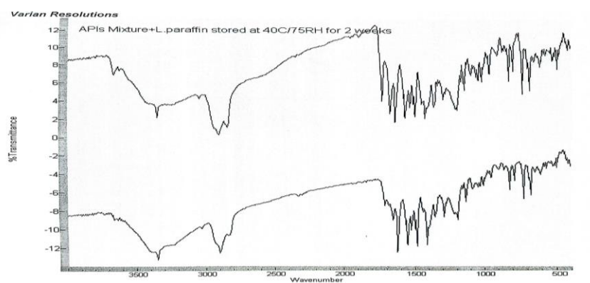
Fig. 13: FTIR Spectra of the API Mixture to the Stored Drug-Excipient Mixture with Liquid Paraffin.
