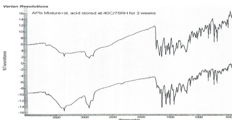
Fig. 12: FTIR Spectra of the API Mixture to The Stored Drug-Excipient Mixture with Stearic Acid.
