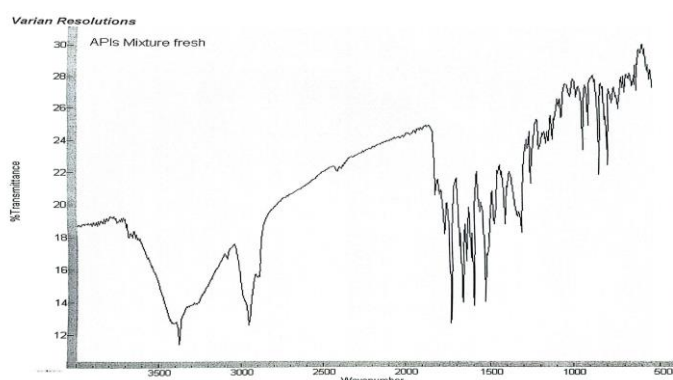
Fig. 3: FTIR Spectra of APIs Mixture.
