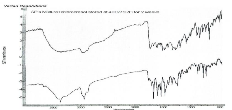
Fig. 9: FTIR Spectra of the API Mixture to the Stored Drug-Excipient Mixture with Chlorocresol.
