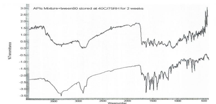
Fig. 8: FTIR Spectra of the API Mixture to the Stored Drugs-Excipient Mixture with Tween 80.
