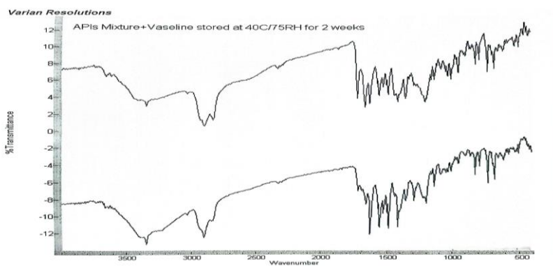
Fig. 7: FTIR Spectra of the API Mixture to the Stored Drug-Excipient Mixture with Vaseline.
