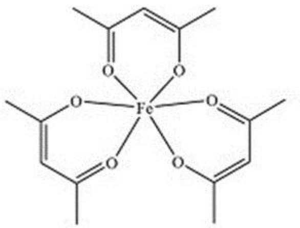
Figure 6: structure Tris(acetylacetonato) iron[III] Single Source Precursor.
